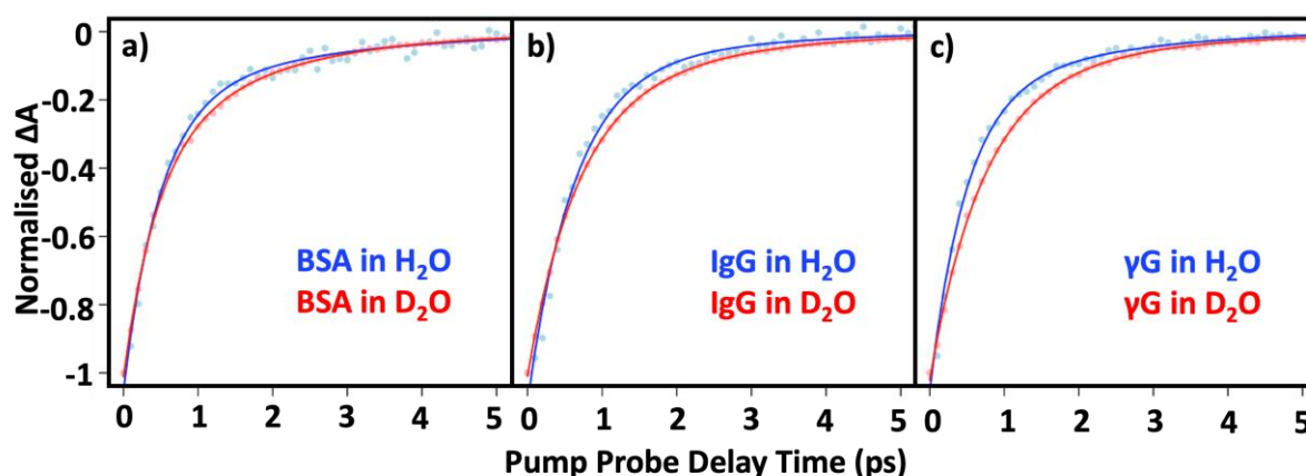
Figure 3: Temporal variation of the amide I v=0-1 transition for (a) BSA (b) Immunoglobulin G and (c) \gamma -globulins in both D_2O (red) and H_2O (blue) solvents. Solid lines denote tri-exponential fits for H_2O and single exponential decays for D_2O . 13
