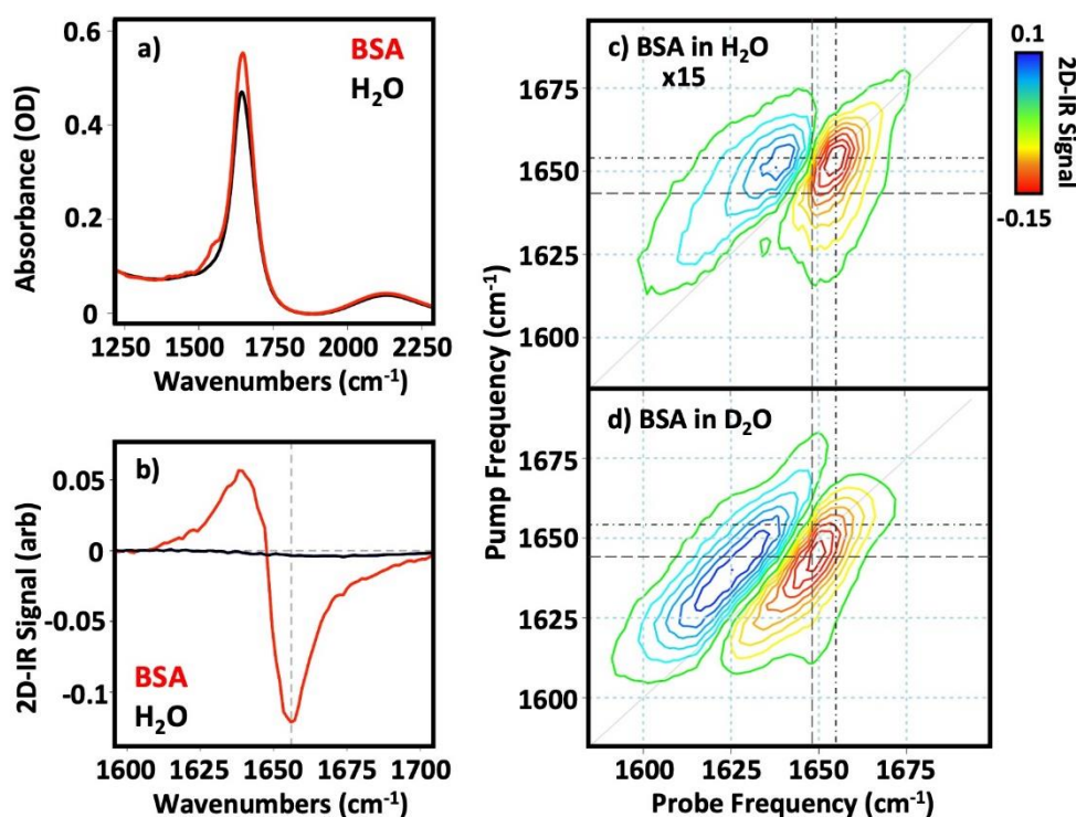
Figure 1: a) FTIR spectra of \text{H}_2\text{O} (black) and a solution of bovine serum albumin (BSA, 30 g/L) in \text{H}_2\text{O} (red). The protein concentration corresponds to \sim 0.45 mM and the sample path length was \sim 3\mu\text{m} b) Pump frequency slice taken from the 2D-IR spectra of \text{H}_2\text{O} (black) and BSA (30 g/L) in \text{H}_2\text{O} (red) at a frequency of 1656\text{ cm}^{-1} . 2D-IR spectra of BSA (30 g/L) shown in both c) \text{H}_2\text{O} with path length \sim 3\mu\text{m} and d) \text{D}_2\text{O} with path length of 25\mu\text{m} . Note c) is scaled by a factor of 15 to enable plotting on similar scale to that of d). 13 All 2D-IR spectra were obtained with a waiting time of 250 fs.
