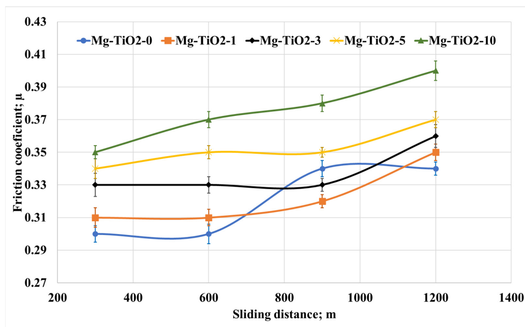
Figure 8. Friction coefficient of Mg/TiO 2 nanocomposites under different sliding distances, 30 N.
