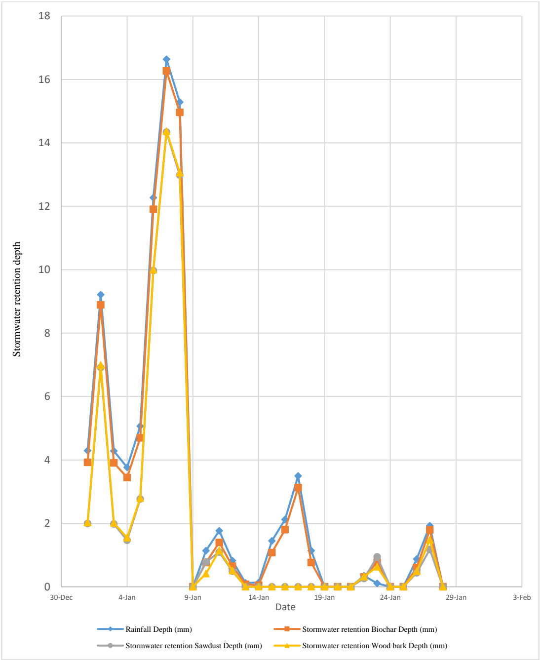
Figure 1: Stormwater runoff depth curve
