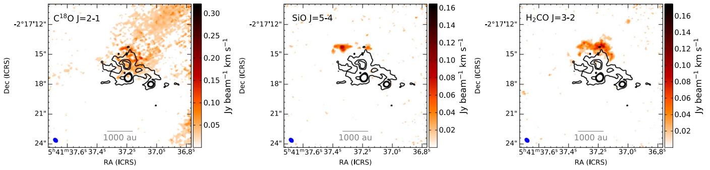
Figure 5. Integrated intensity maps of C^{18}O , SiO, and H_2CO emission, with the dust continuum in black contours at 3\sigma_{1.3 \text{ mm}} , 10\sigma_{1.3 \text{ mm}} , and 20\sigma_{1.3 \text{ mm}} .
