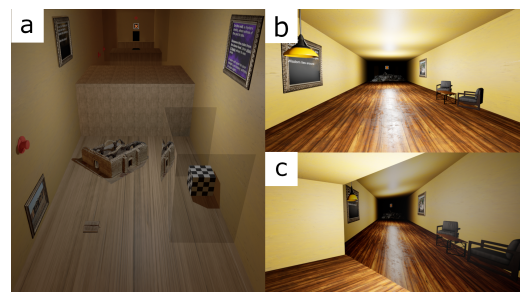
Figure 4: Gravity (a) and deception (b, c) optical illusions.
