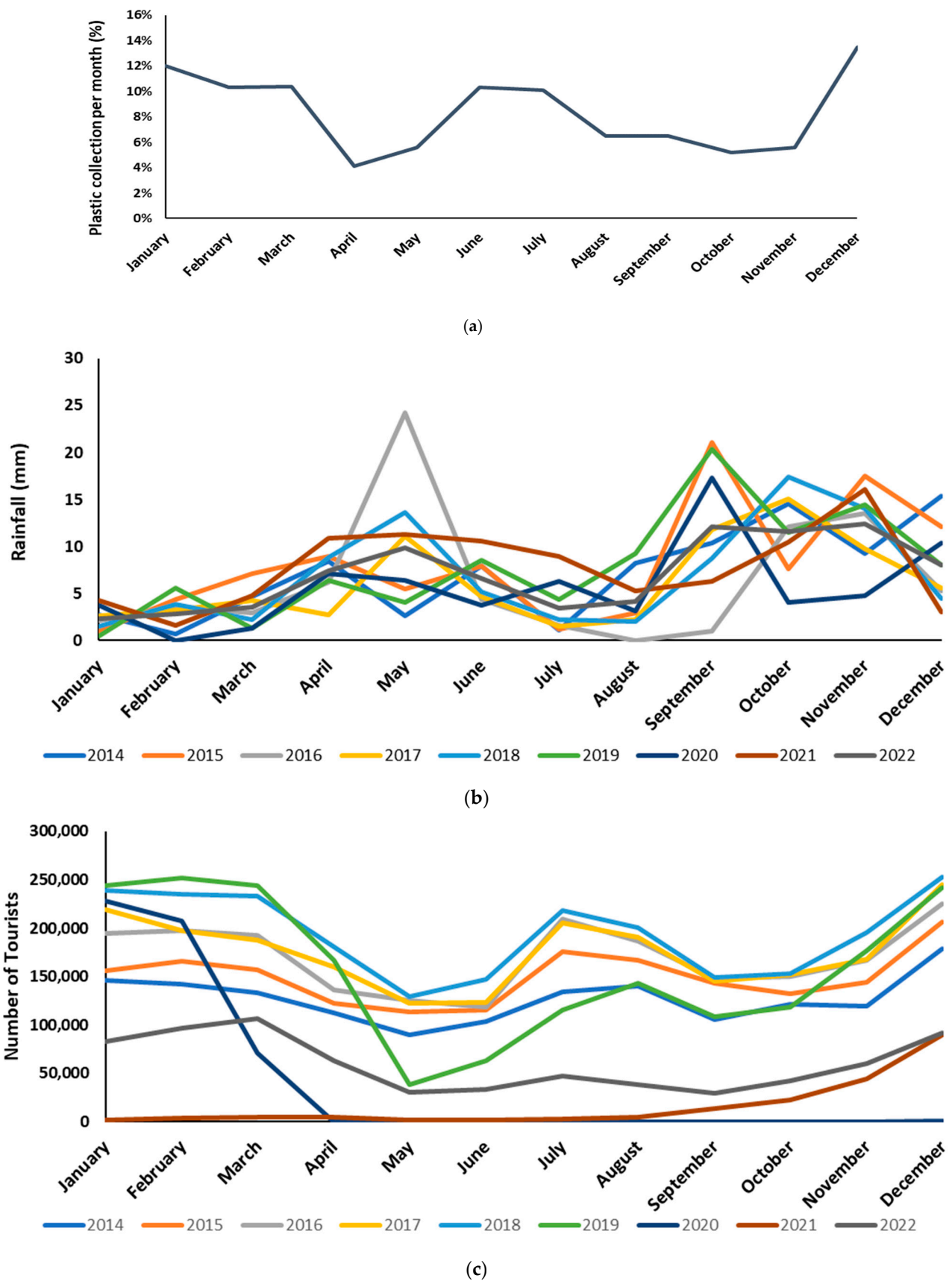
Figure 6. Correlation between (a) monthly plastic waste received, (b) rainfall patterns, and (c) tourist arrivals in Sri Lanka over the past 9 years.
