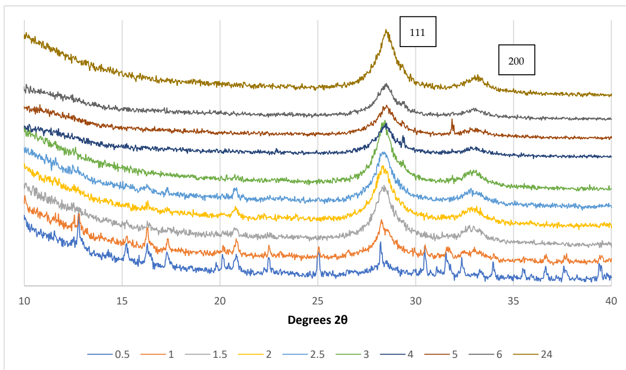
Figure 2. Variation in \text{CeO}_2 film peak formed with calcination time (in h, see figure legend) at 200 \text{ }^\circ\text{C} . Shortest times at the bottom of the graph. No post-processing was applied to these data beyond cropping.
