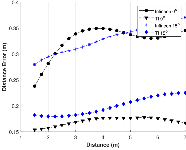
Fig. 7. Infineon versus TI distance accuracy.
