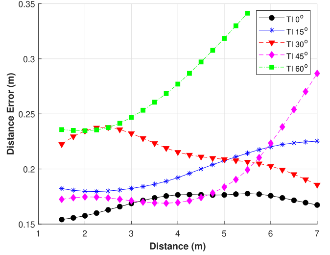
Fig. 8. IWR1642BOOST distance accuracy.
