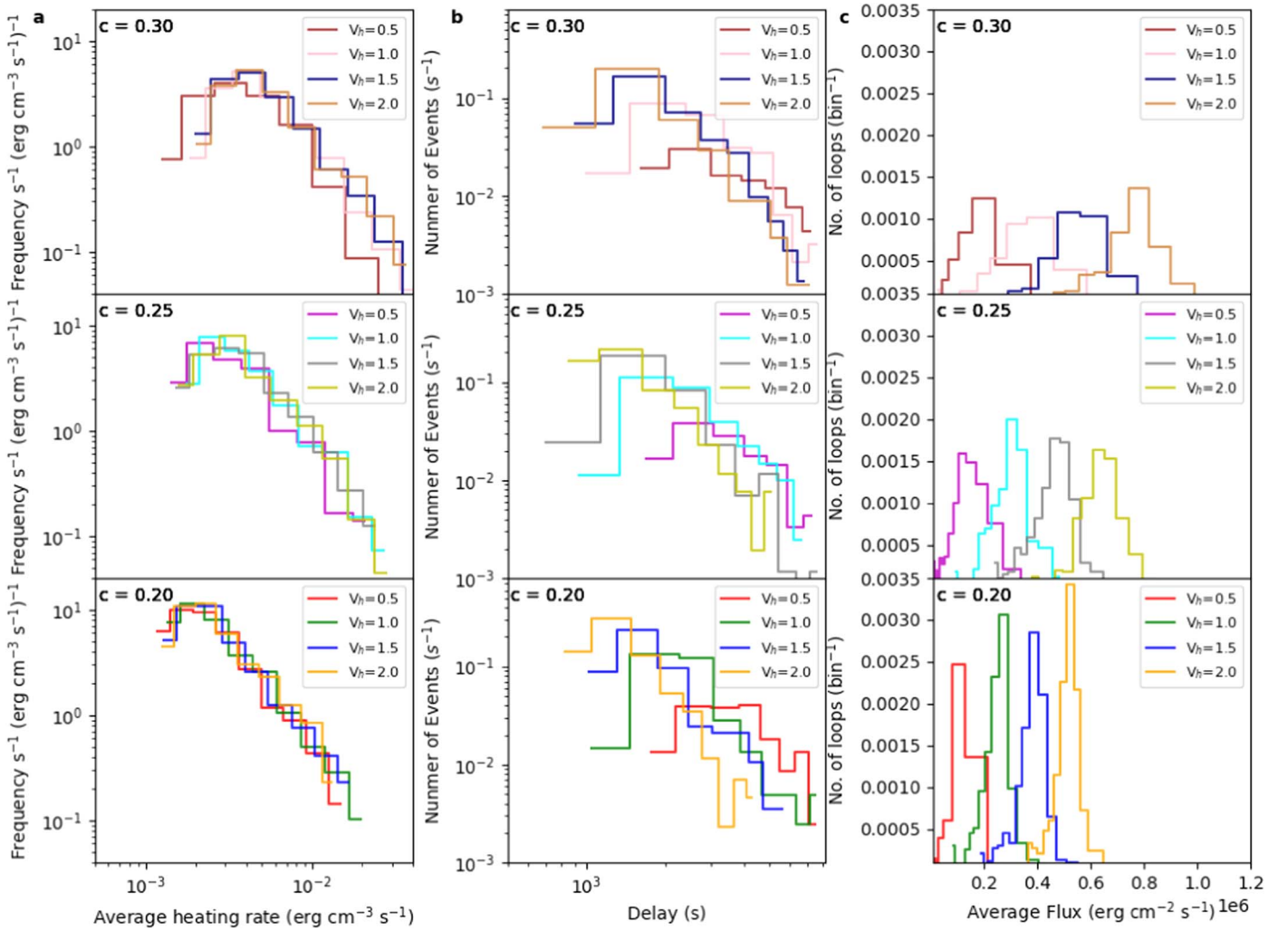
Figure 4. The variation of the composite distribution of heating events for different heating parameters. Panel (a) shows the average frequency distribution for all the loops as a function of heating rate. Panel (b) shows the distribution of the delay time between successive events for all the loops, where the average delay for each distribution is labeled. Panel (c) shows the distribution of the average Poynting flux for all the loops.
