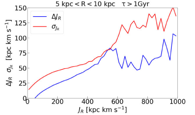
Figure 18. The heating, \Delta J_R = \langle J_R \rangle_t - J_R (blue), and the instantaneous radial action measurement uncertainty, \sigma_{J_R} , computed as the standard deviation of (J_R - \langle J_R \rangle_t) (red). Only stars older than 1 Gyr in the disc are considered. See the text for why \Delta J_R overestimates the heating.
