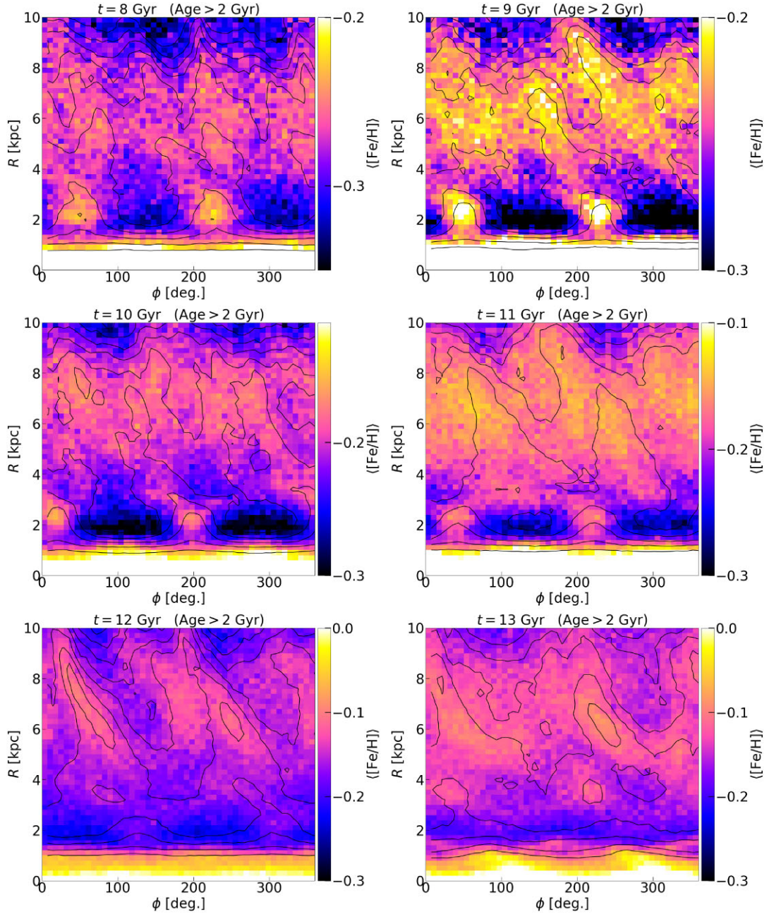
Figure A1. [Fe/H] in cylindrical coordinates at t = 8 – 13 Gyr, as labelled. Only stars older than 2 Gyr are considered (compare Fig. 1). The contours correspond to the full surface density. Note the changing colour scale.
