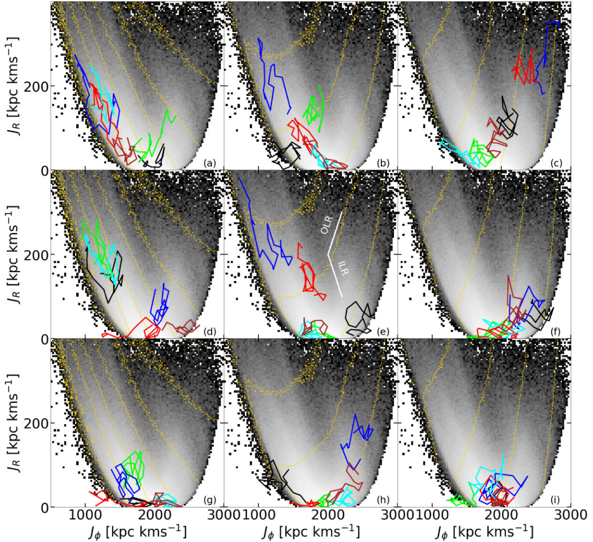
Figure 26. The evolution of a random set of 54 particles, selected as described in the text, in the action space (J_\phi, J_R) . In each panel, we present six stars with different colours over a 1 Gyr time interval plotting every 50 Myr. The plotted particles are ordered by age, with the oldest in the top row ( 9.2 \leq \tau / \text{Gyr} \leq 11.7 ), the intermediate-age ones in the middle row ( 4.7 \leq \tau / \text{Gyr} \leq 8.8 ) and the youngest in the bottom row ( 2.2 \leq \tau / \text{Gyr} \leq 4.2 ). The dashed yellow lines show contours of constant E_J for \Omega_p = 15.4 \text{ km s}^{-1} \text{ kpc}^{-1} (left panel), 40.0 \text{ km s}^{-1} \text{ kpc}^{-1} (centre panel), and 61.5 \text{ km s}^{-1} \text{ kpc}^{-1} (right panel). The white lines in panel (e) indicate the libration vectors at the OLR (upper line) and the ILR (lower line). The background shows a log scale representation of the number density of stars.
