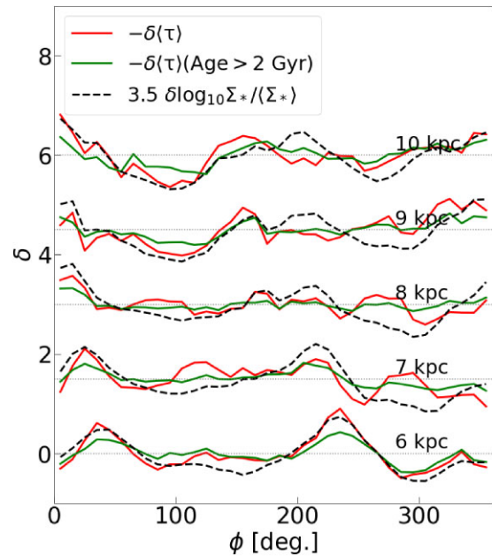
Figure 12. The variation of \langle \tau \rangle compared with the density variation at a series of 500 pc-wide annuli centred at 6 to 10 kpc, as indicated. (We use -\langle \tau \rangle to permit easier comparison with the density.) The average value at each radius is subtracted from each azimuthal profile and the profiles are then vertically offset by a fixed amount to show the variation. The azimuthal profiles of the density have been scaled by the factor 3.5 for ease of comparison. The dotted horizontal lines indicate the zero for each radius. The red (green) lines show \langle \tau \rangle profiles of all stars (stars older than 2 Gyr).
