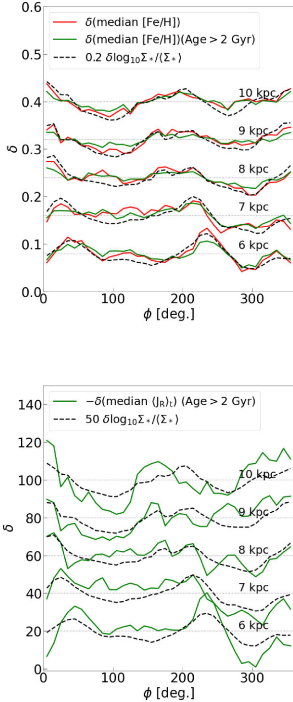
Figure B2. The variation of median [Fe/H] (top panel) and -\text{median} \langle J_R \rangle_t (bottom panel) compared with the density variation at a series of 500 pc-wide annuli centred at 6 to 10 kpc, as indicated. The average value at each radius is subtracted from each azimuthal profile and the profiles are then vertically offset by a fixed amount to show the variation. The azimuthal profiles of the density have been scaled for ease of comparison. The dotted horizontal lines indicate the zero for each radius. In the top panel, the red lines show profiles of median [Fe/H] for all stars, while the green lines show stars older than 2 Gyr only (both panels). Compare these with Fig. 2 and the right panel of Fig. 15.
