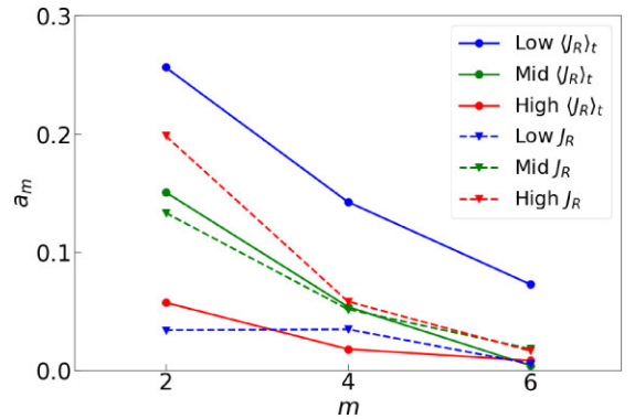
Figure 19. The m = 2, 4, and 6 Fourier amplitudes of the density distribution at 5.5 < R/\text{kpc} < 6.5 separated into equal-sized low, medium and high populations of \langle J_R \rangle_t (solid lines) and J_R (dashed lines).
