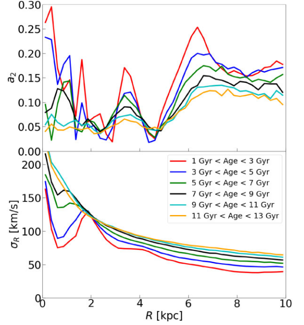
Figure 10. Top panel: the radial profiles of the amplitude of the m = 2 density Fourier moments for different age populations, as indicated in the legend. Outside 5 kpc, spiral structure is weaker in old populations than in younger ones. Bottom panel: the radial velocity dispersion, \sigma_R , profiles of the same stellar populations. Stars younger than 1 Gyr are not plotted.
