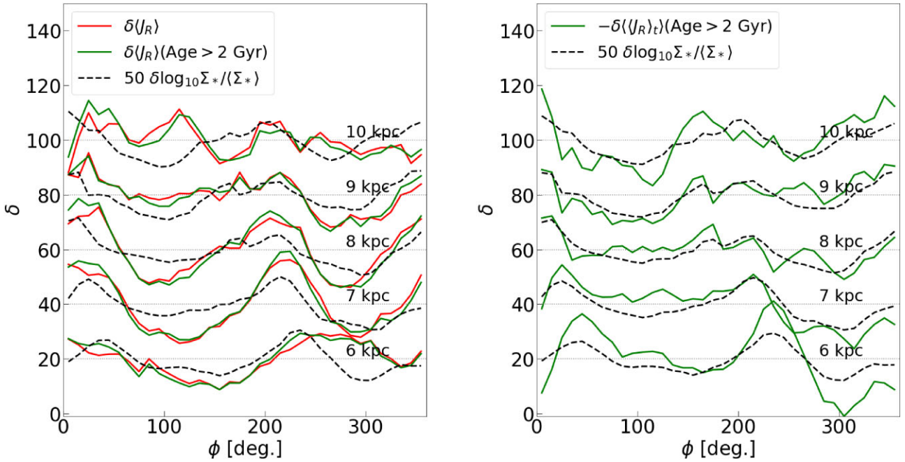
Figure 15. The variation of \langle J_R \rangle (left panel) and -\langle J_R \rangle_t (note the sign difference) compared with the density variation at a series of 500 pc-wide annuli centred at 6 to 10 kpc, as indicated. The average value at each radius is subtracted from each azimuthal profile and the profiles are then vertically offset by a fixed amount to show the variation. The azimuthal profiles of the density have been scaled by the factor 50 for ease of comparison. The dotted horizontal lines indicate the zero for each radius. The red lines show \langle J_R \rangle profiles of all stars (left panel), while the green lines show stars older than 2 Gyr only (both panels).
