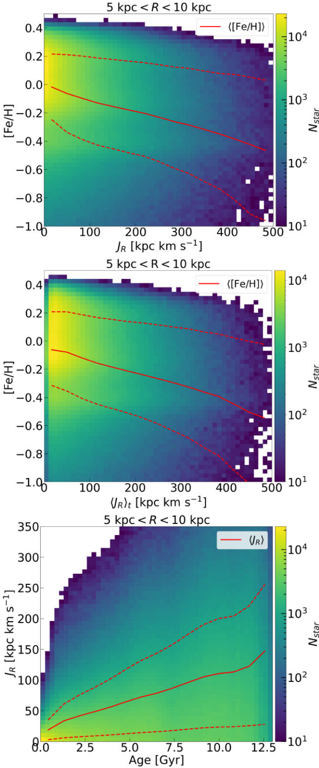
Figure 13. The J_R -[Fe/H] (top panel), \langle J_R \rangle_t -[Fe/H] (middle panel), and \tau - J_R relations (bottom panel) for star particles at 5 \leq R/\text{kpc} \leq 10 at 13 Gyr. The solid lines show \langle[\text{Fe}/\text{H}]\rangle (top and middle panels) and \langle J_R \rangle (bottom panel). In all panels, the dashed curves show the 16 and 84 per cent distributions. The middle panel excludes stars younger than 2 Gyr, which results in the paucity of low \langle J_R \rangle_t stars.
