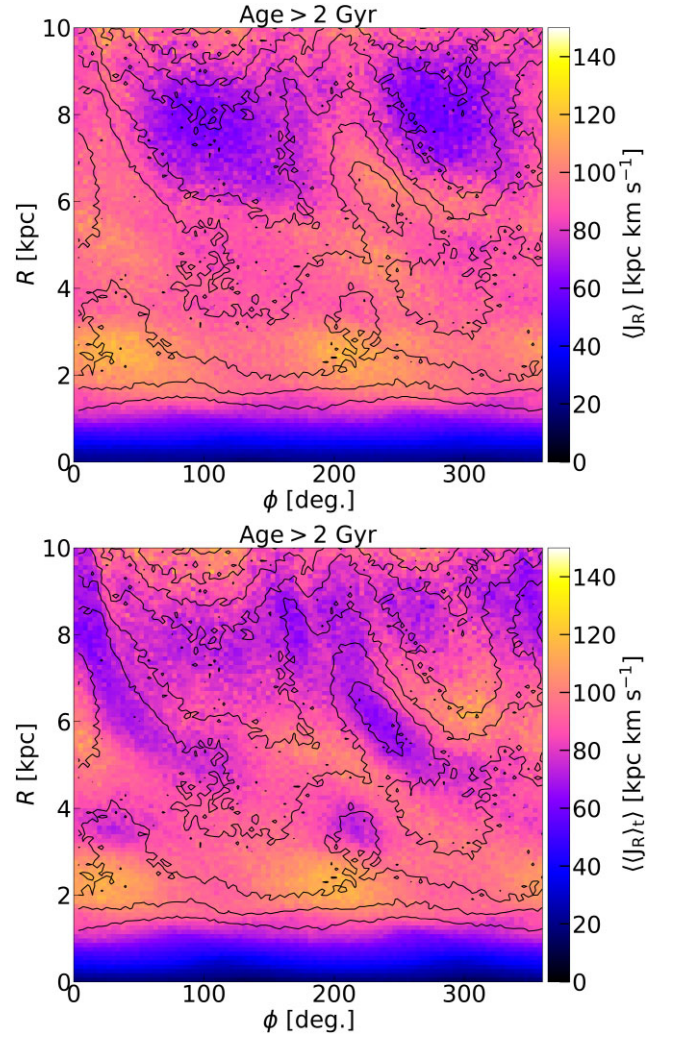
Figure 14. The mean instantaneous radial action, \langle J_R \rangle , (top panel) and the mean time-averaged radial action, \langle \langle J_R \rangle_t \rangle , (bottom panel) in cylindrical coordinates. The contours correspond to the surface density. Only stars older than 2 Gyr have been considered. The disc is rotating in a counter-clockwise sense, i.e. rotation is in the direction of increasing \phi . The model is shown at 13 Gyr.
