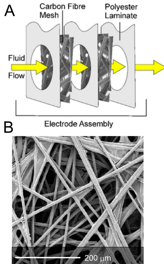
Figure 3. (A) Carbon fiber electrode configuration and (B) scanning electron image of the Toray carbon fiber mesh.
