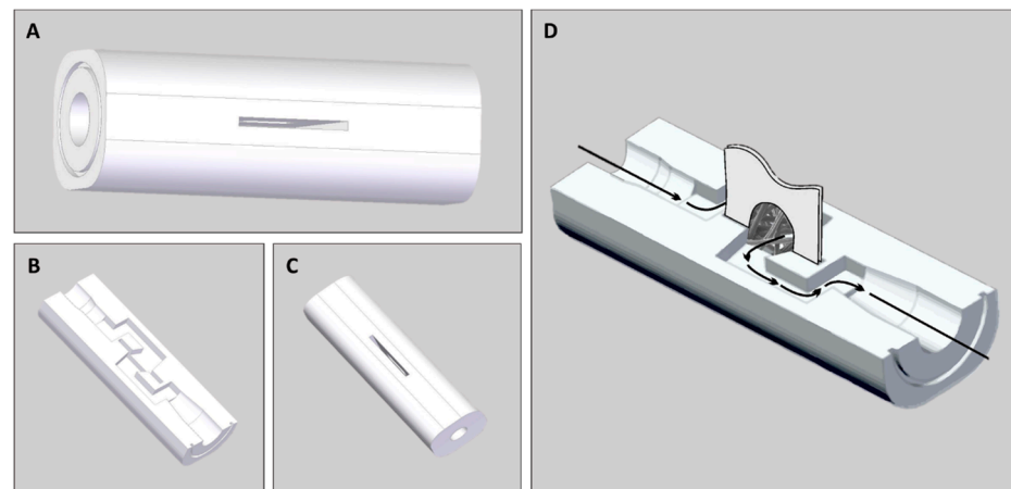
Figure 4. Schematics highlighting the external (A,C) and internal (B) design of the needle-free hub and the proposed flow path (D).
