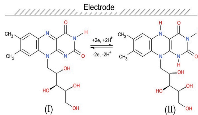
Figure 2. Electrochemical redox transitions of riboflavin at an electrode detailing the reduction (I → II) and corresponding oxidation (II → I).
