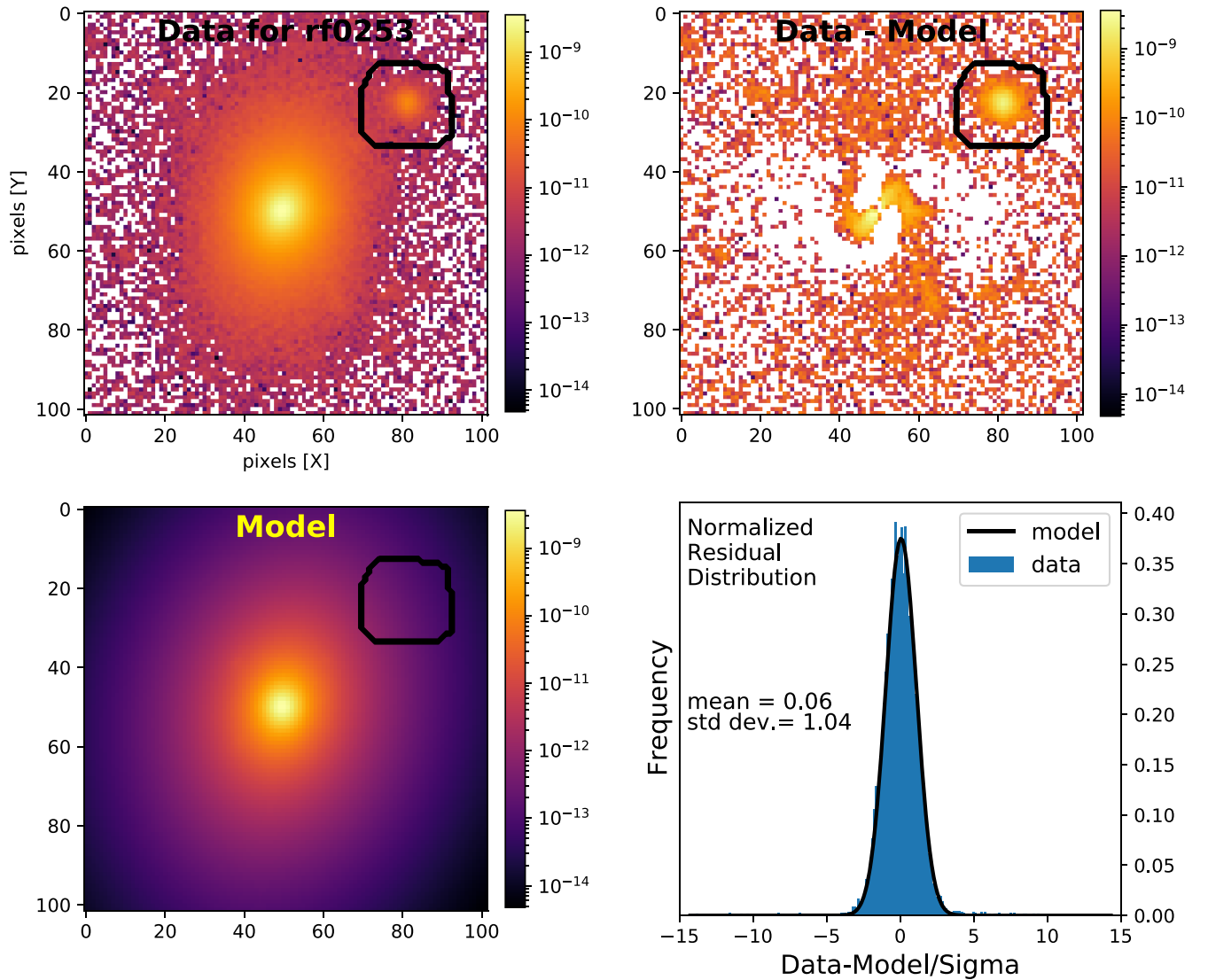
Figure 1. Data, model, and residual images for the PyProFit single-Sérsic model of RESOLVE galaxy rf0253. The x -axis and y -axis for the images are in units of pixels, and the color bar is in units of maggies. In this figure, the black contour denotes a region excluded from the fitting process. The bottom-right subplot is the distribution of the residuals of the fitted pixels normalized to the flux uncertainty value, \sigma . A Gaussian model fit (black line and inset statistics) indicates residuals only slightly exceed the uncertainty. A spiral structure is revealed in the residual subplot. This figure replicates the analysis of ProFit models in Moffett et al. (2019).
