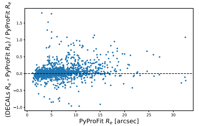
Figure 3. Comparison of \text{PyProFit } R_e and \text{DECaLS } R_e for galaxies in the parent survey that have both estimates. The dashed line marks where the fractional difference between estimates is zero. The median value for the data on the y-axis is 0.01 and the standard deviation is 0.24, suggesting strong agreement between the two radius estimates.
