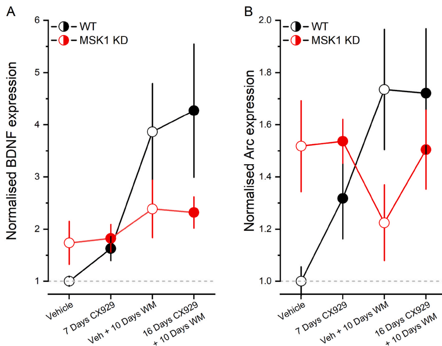
Fig. 5. Influence of MSK1 on BDNF and Arc expression as a function of experience and ampa-kine treatment. A) BDNF expression across treatments and genotypes relative to expression in 7-day vehicle-treated WT mice from Fig. 4A. BDNF expression showed an appreciable classic sigmoidal dose-response relationship in WT mice, whereas in MSK1 KD mice the range of expression was greatly reduced. B) Arc expression across treatments and genotypes relative to expression in 7-day vehicle-treated WT mice from Fig. 4B. In contrast to the strong dose-response relationship in WT mice, Arc expression in the MSK1 KD mice showed no relationship to experience or ampa-kine treatment. Data are expressed as mean \pm SEM.
