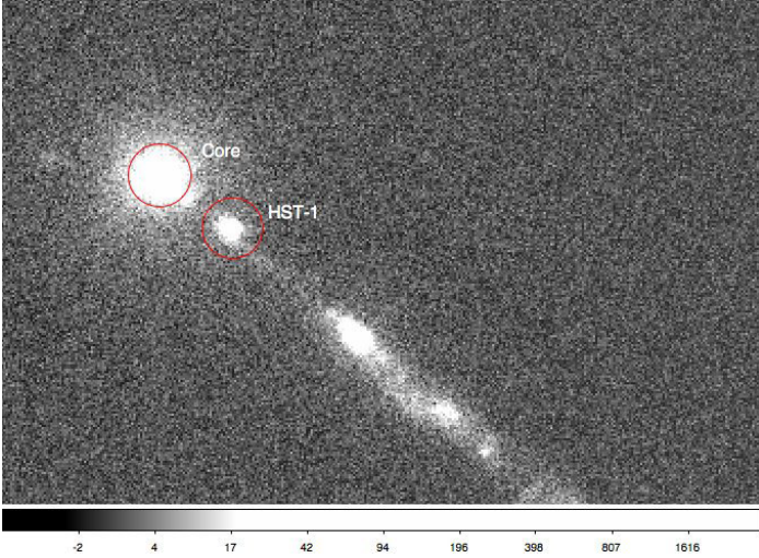
Fig. 5. Hubble Space Telescope image of M87 at 2359.7 Å with the host galaxy subtracted. The core and HST-1 are indicated; the distance between the features is 1^{\prime}00 \pm 0^{\prime}05 , and the pixel size is 0^{\prime}0248 .
