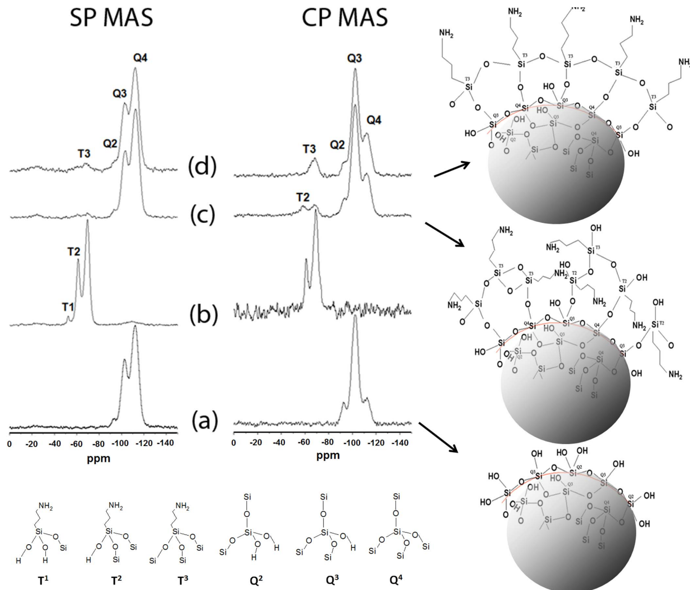
Figure 3 | ^{29}\text{Si} single pulse (SP) and ^{29}\text{Si} - ^1\text{H} cross polarization (CP) magic angle sample spinning (MAS) spectra of non-aminosilanes diamagnetic silica nanoparticles. (a); condensed/polymerised APTS (b); silica nanoparticles aminosilanes in water (c) and silica nanoparticles aminosilanes via TPPE (d).
