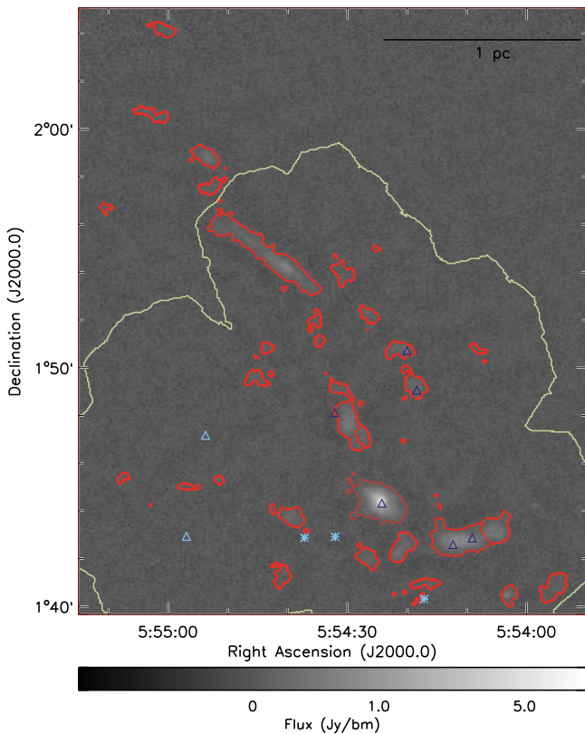
Figure 5. Dense cores identified in L1622. The background grayscale image shows the SCUBA-2 850 \mu\text{m} emission. The red contours show the dense core boundaries, as identified with FellWalker, while the blue triangles show locations of protostars from the Spitzer YSO catalog of Megeath et al. (2012) and blue asterisks show the Herschel YSO catalog of Stutz et al. (2013). Dark symbols indicate protostars associated with a dense core, while light symbols indicate unassociated protostars. The light yellow contour denotes the Herschel coverage for the Stutz et al. (2013) catalog (A. Stutz 2015, private communication).
