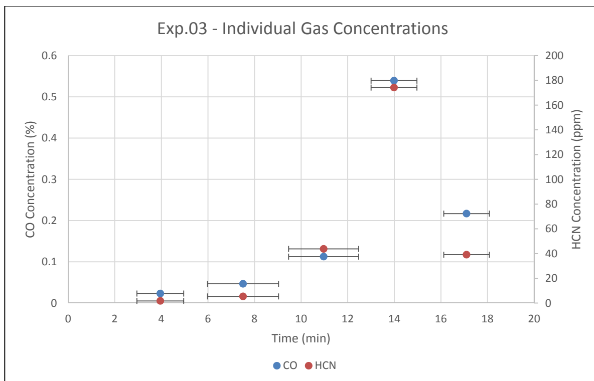
Figure A8 – Experiment 03 individual gas concentrations
