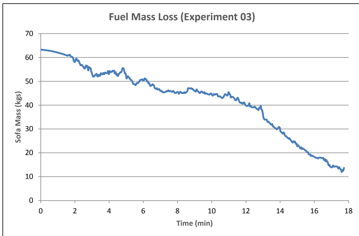
Figure 69 – Experiment 03 mass loss corrected readings
