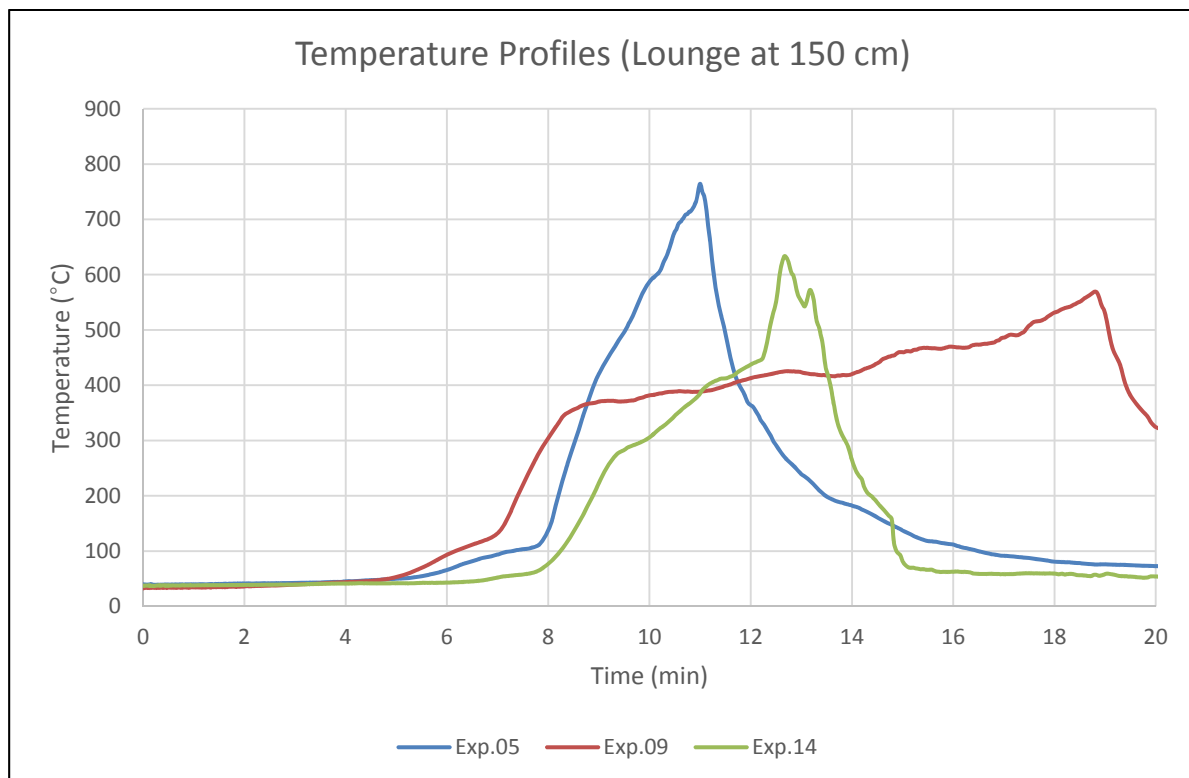
Figure 93 – Lounge closed door temperature profiles (lounge at 150 cm)
