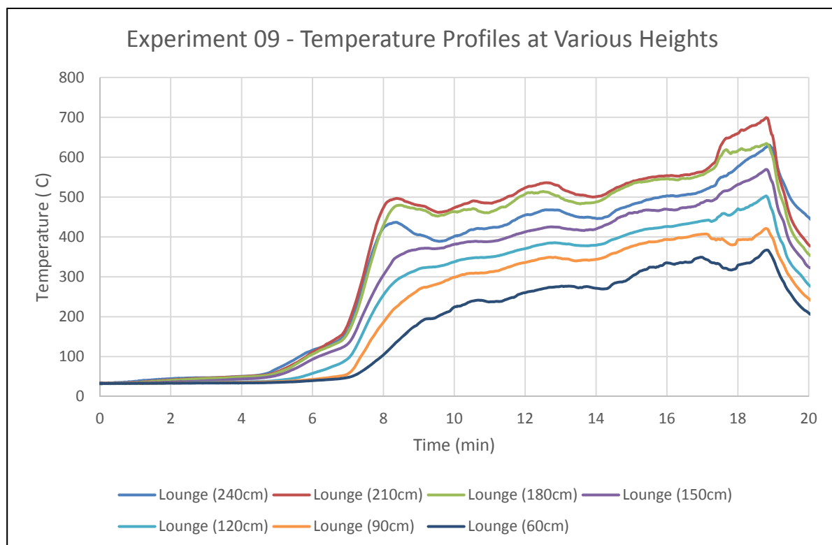
Figure 97 – Experiment 09 lounge temperature profiles (at various heights)
