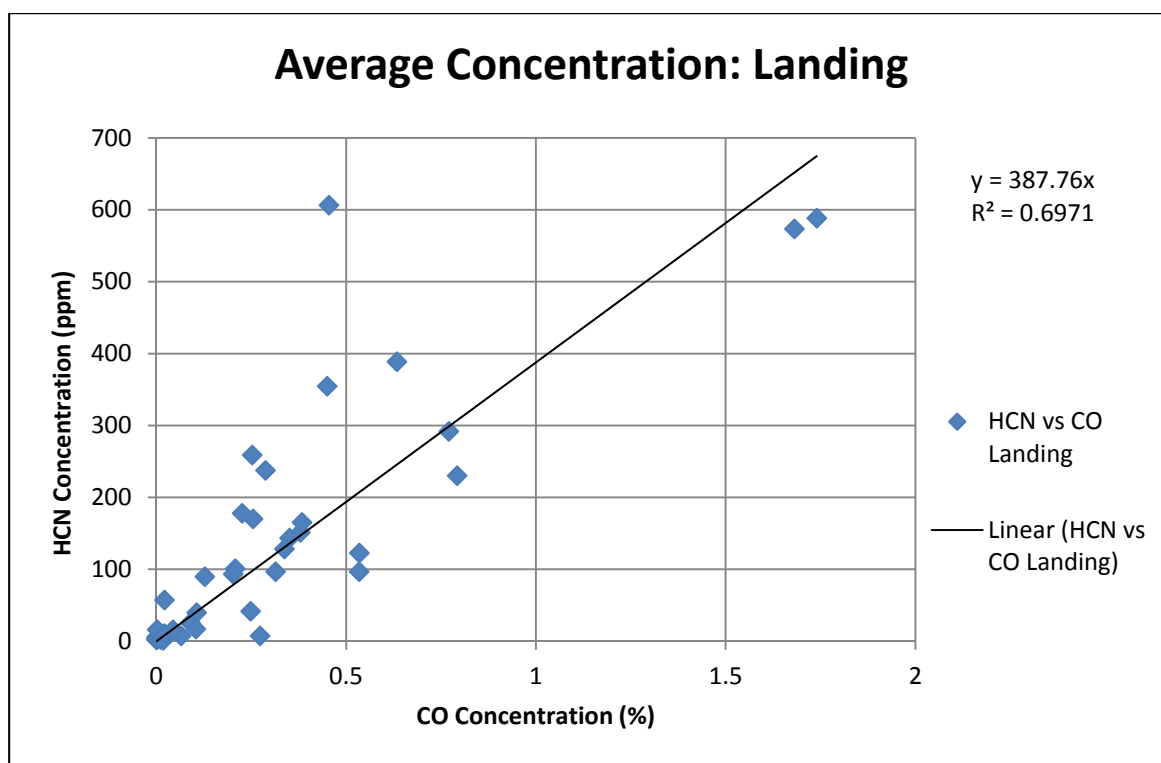
Figure 55 – CO to HCN equivalence ratio (landing)
