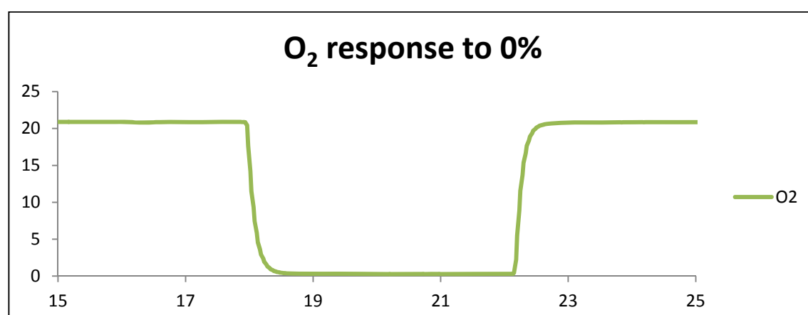
Figure A7 – O 2 calibration response to 0.0% oxygen
