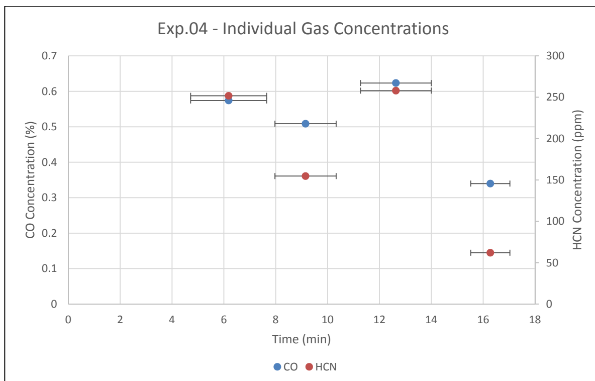
Figure A9 – Experiment 04 individual gas concentrations
