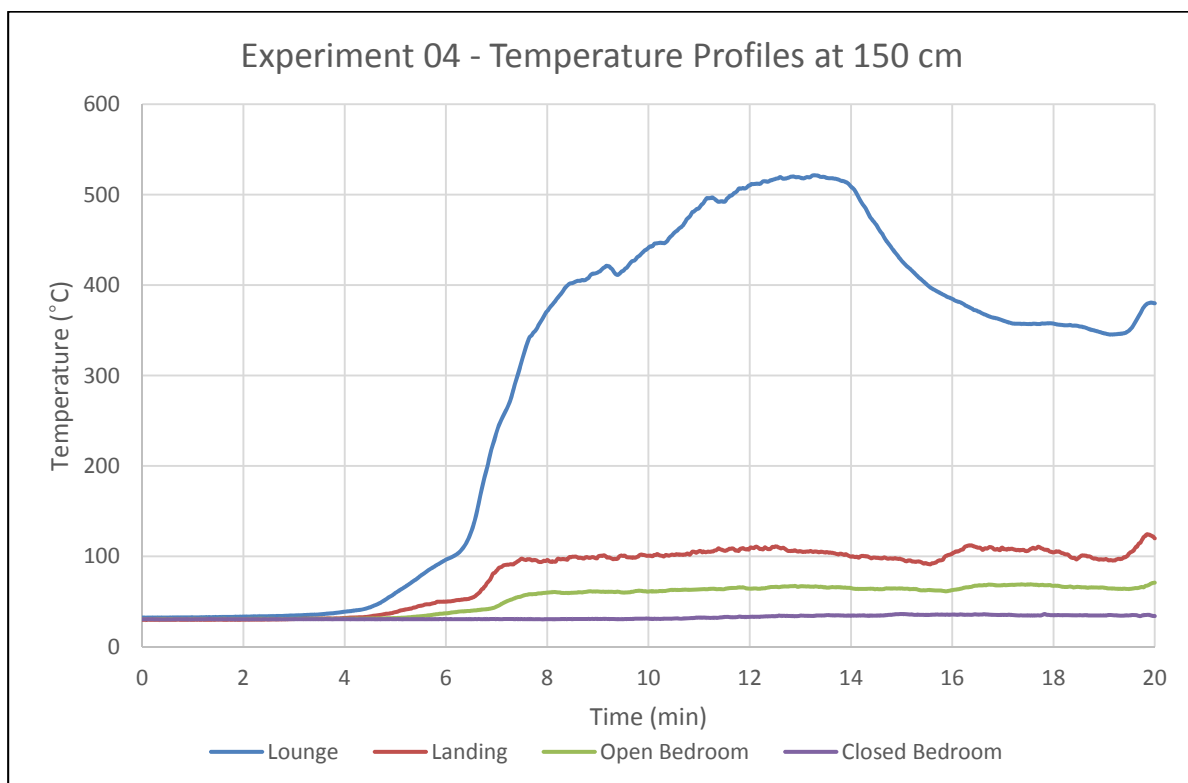
Figure 63 – Experiment 04 temperature profiles (at 150 cm)
