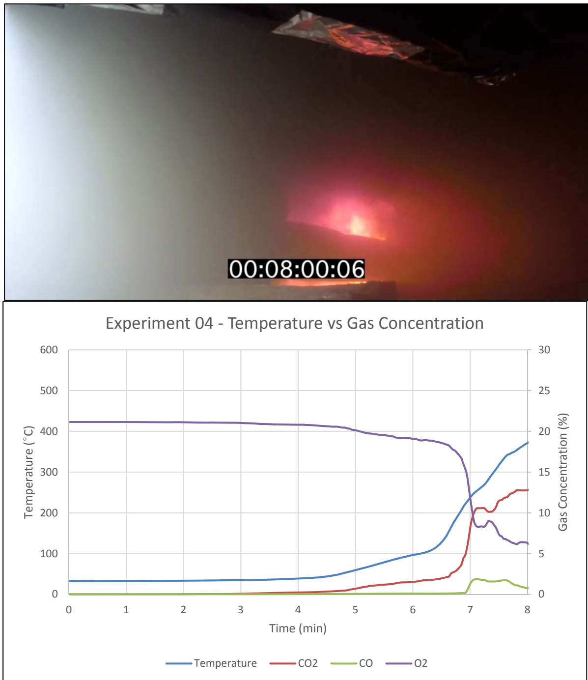
Figure 84 – Experiment 04 – temperature/gas concentrations vs time (8 min)
