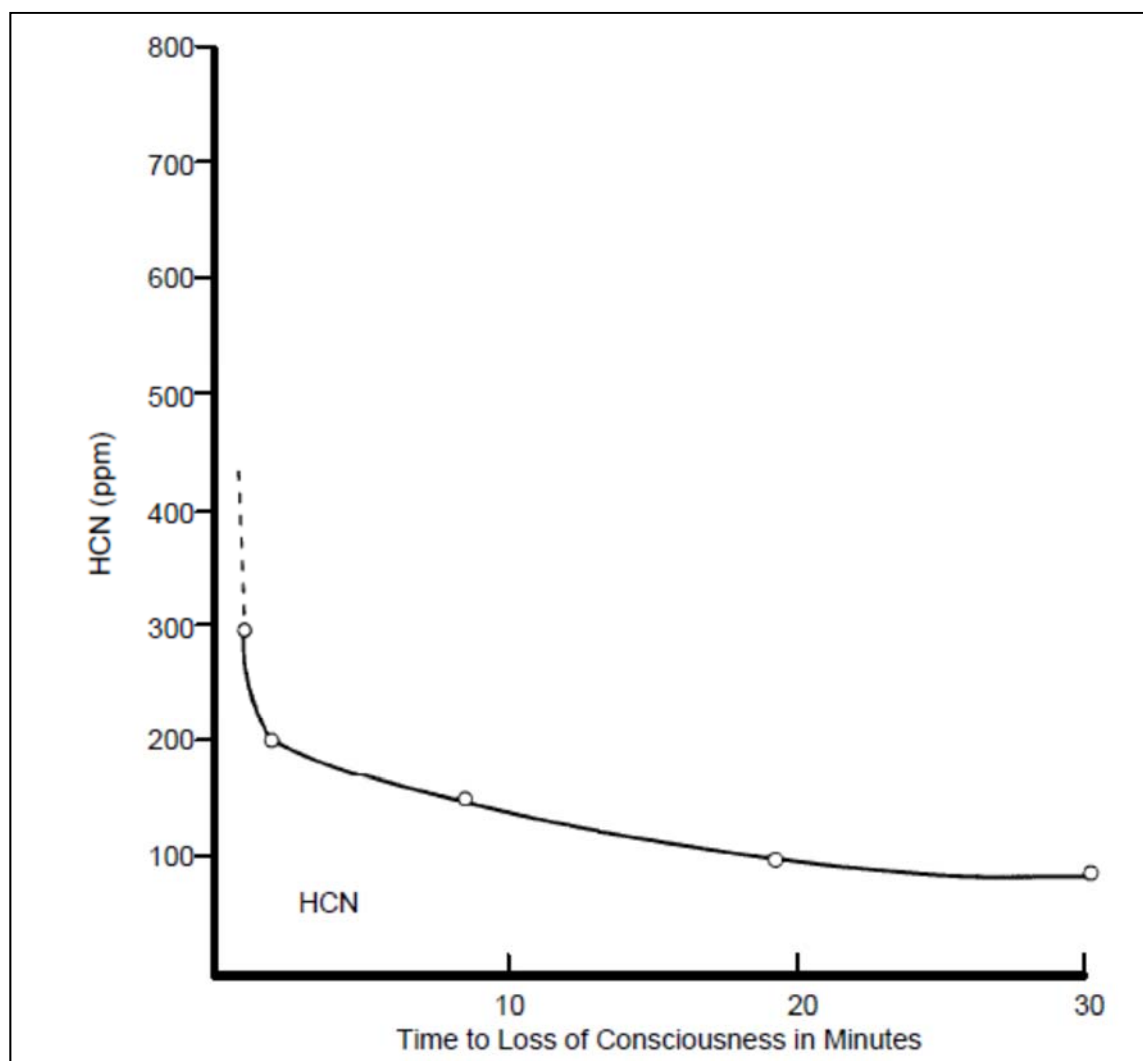
Figure 4 – Time to incapacitation for seated monkeys exposed to HCN [36]
