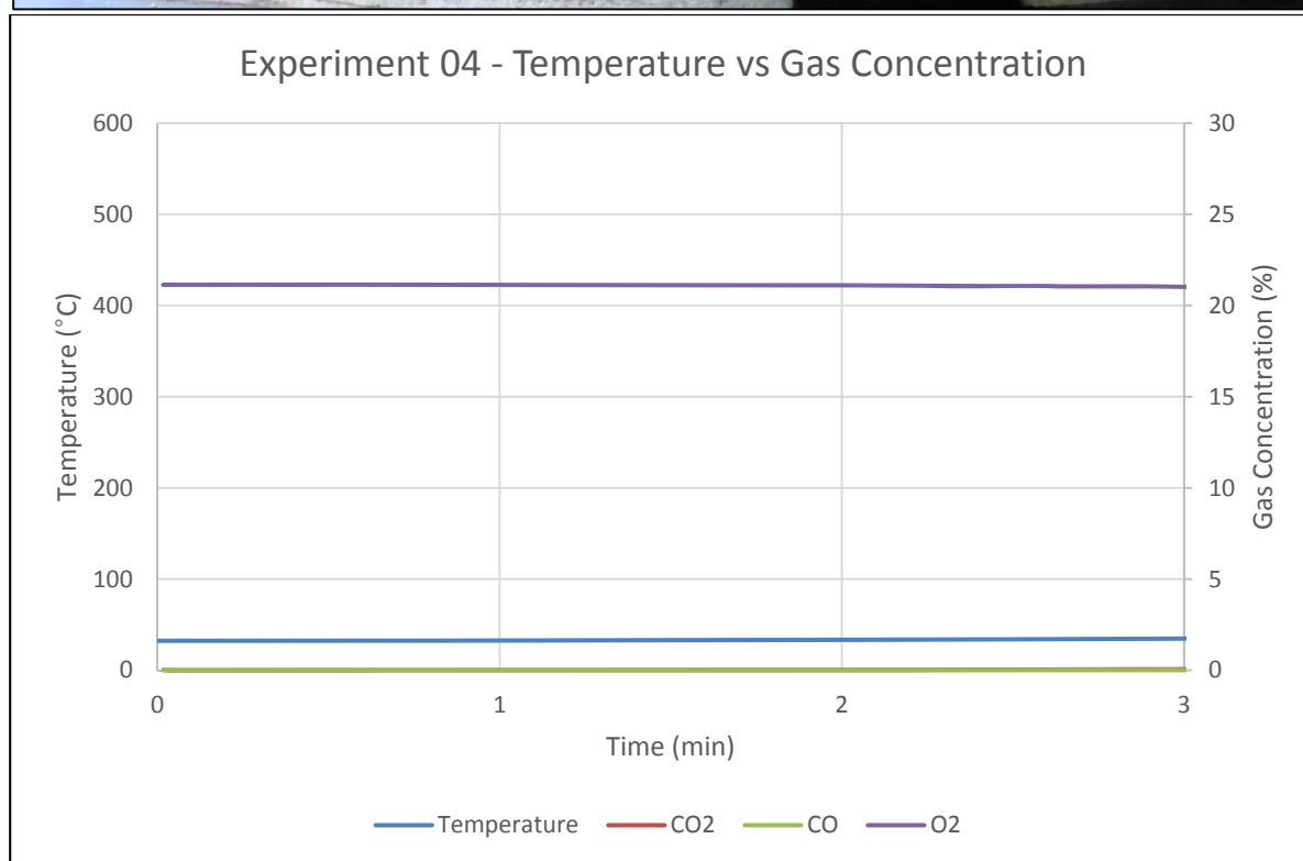
Figure 79 – Experiment 04 – temperature/gas concentrations vs time (3 min)
