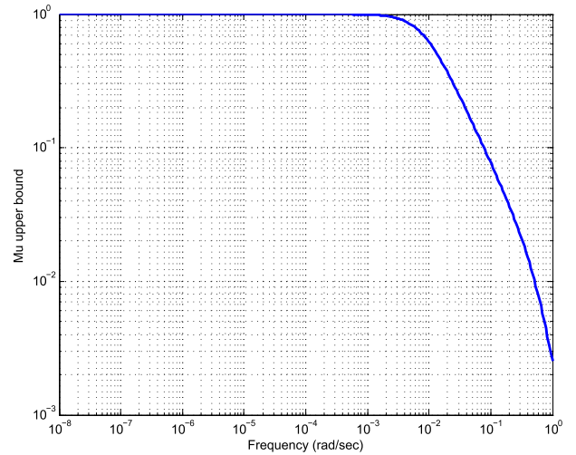
FIGURE 4. Upper bound of the structured singular value \mu of linear system (supplementary file S6) with y_{15} as input.
