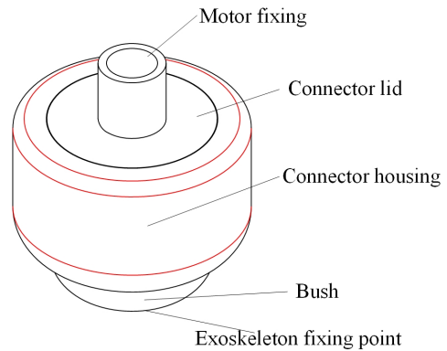
Fig. 3 Connector
