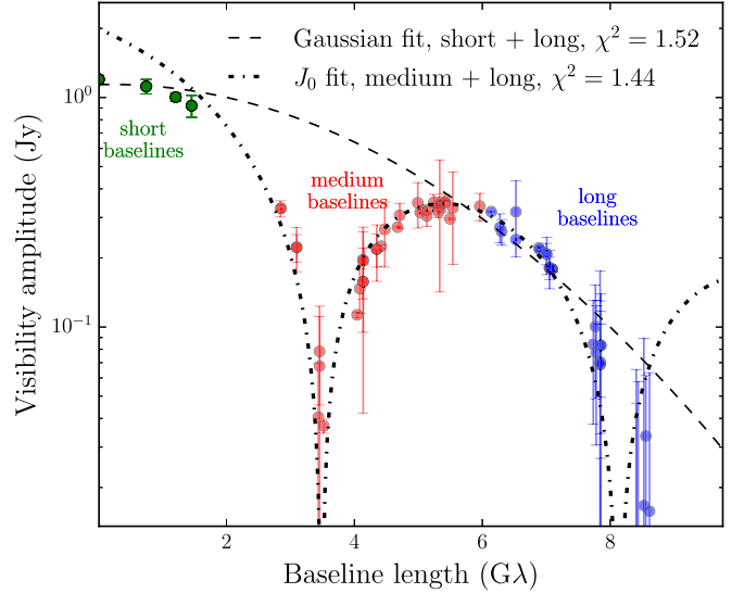
Figure 4. Visibility amplitudes of a simulated 2017 EHT observation of a ring ( 25 \mu\text{as} radius, 5 \mu\text{as} width, convolved with 10 \mu\text{as} circular Gaussian) are shown as a function of radial baseline length \rho . Short ( \leq 2 \text{ G}\lambda ), medium ( 2 \text{ G}\lambda < \rho < 6 \text{ G}\lambda ), and long ( \geq 6 \text{ G}\lambda ) baselines are displayed in green, red, and blue, respectively. Continuous fits of different (but equally well-fitting) models are overlaid. Fitting a ring model with infinitesimal thickness (denoted by J_0 , representing a zeroth-order Bessel function of the first kind) to only medium and long baselines accurately represents the source shape and size but poorly constrains the total intensity of 1 Jy. In addition, an equally good fit can be obtained with a simple Gaussian fit to only short and long baselines. Data from all three baseline types are required to correctly constrain key properties of the source. This result highlights how model misspecification can lead to severe systematic errors, especially when working with limited baseline coverage.
