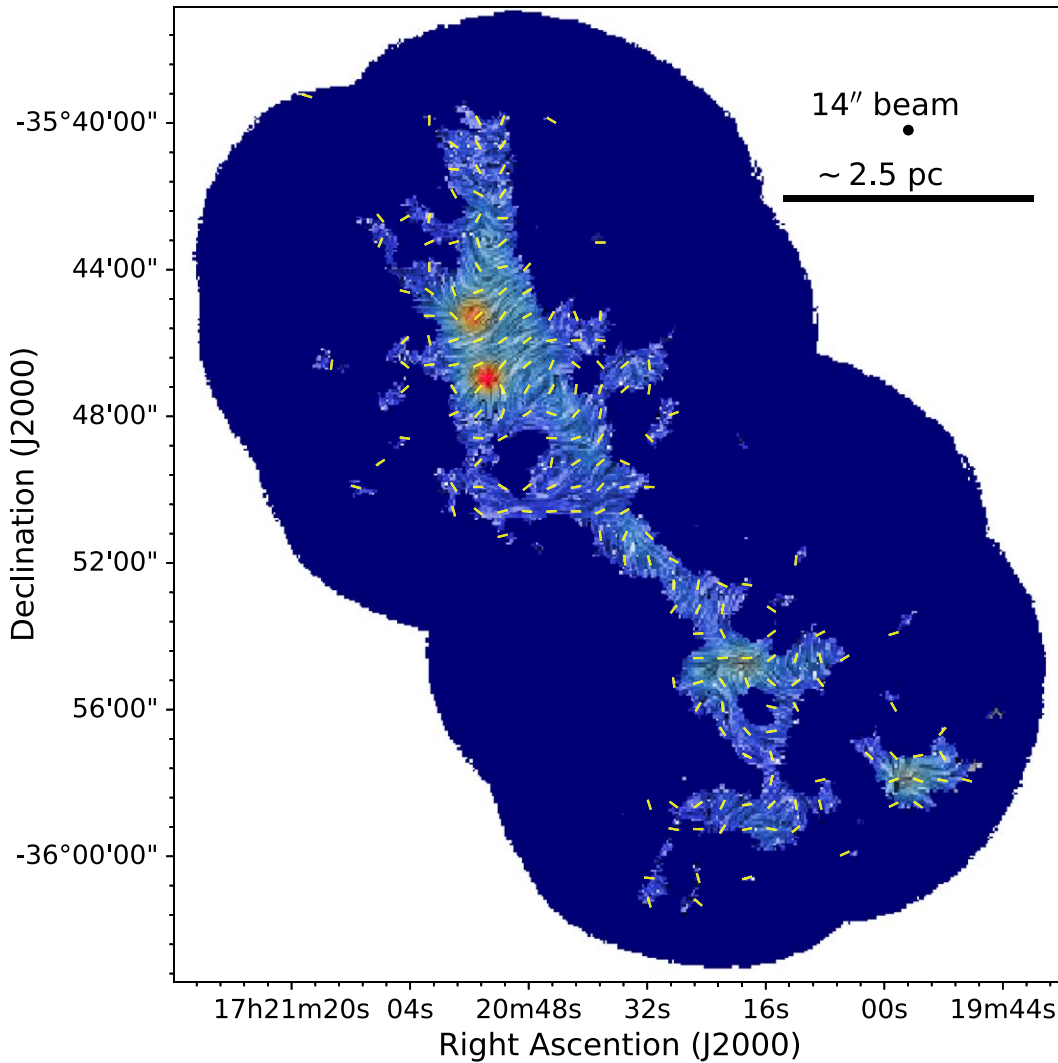
Figure 2. Magnetic field lines associated with NGC 6334 at 850\ \mu\text{m} . The background color image illustrates the Stokes I map, and the drapery lines depict the plane-of-sky magnetic field lines in this region as obtained using the line integration convolution technique. The short yellow lines represent the B_{\text{POS}} orientations (all of the same length), every 10 pixels.
