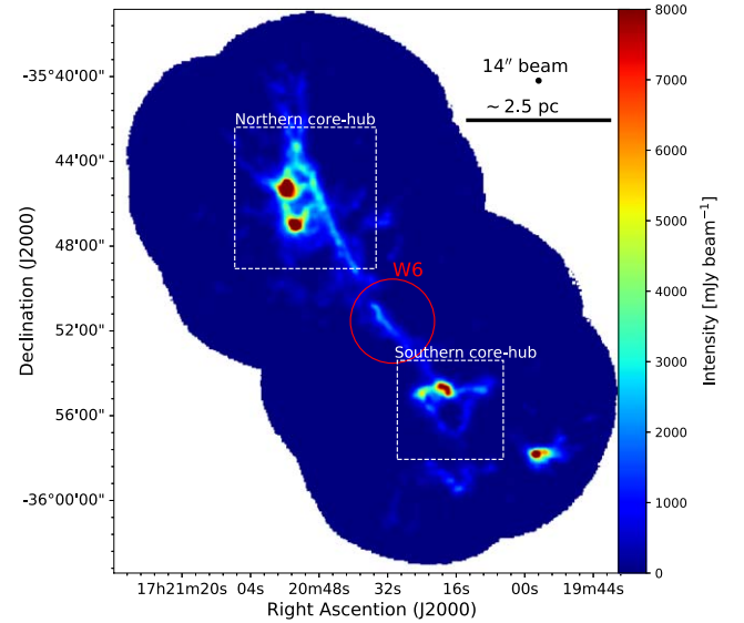
Figure 11. Two dense star-forming regions within NGC 6334, each containing a number of cores. W6 is bounded on both sides by the two core-hub systems.
