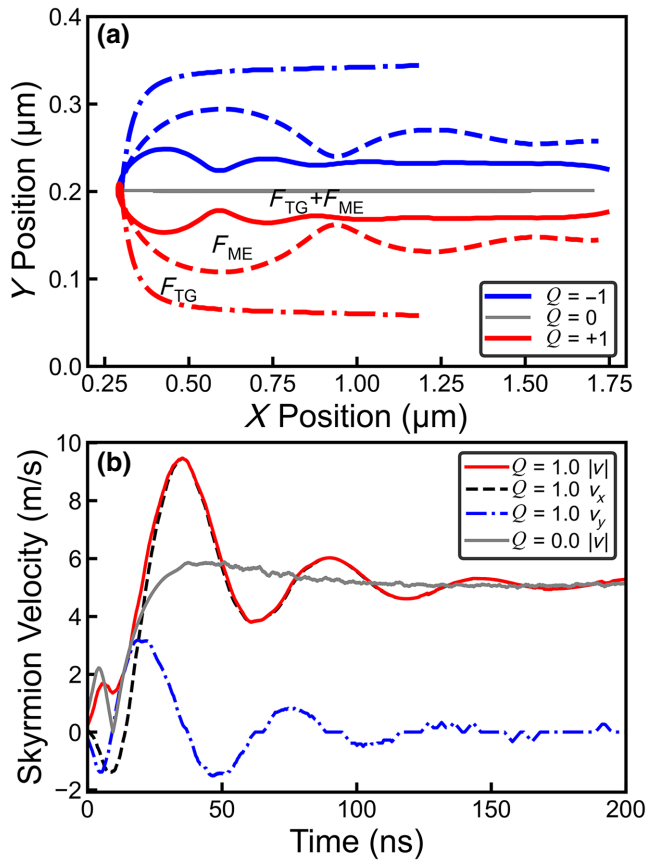
FIG. 2. (a) Computed skyrmion paths for 1-mW absorbed power, with laser spot scanned at 5 m/s through the center of a track 400 nm wide and 2 μm long, shown for ferromagnetic skyrmions ( Q = \pm 1 ) and antiferromagnetic skyrmion ( Q = 0 ). The dash-dot lines show the skyrmion motion without the ME effect, with the resultant motion dependent on the force arising from temperature gradients, F_{TG} , and the effective force due to the Magnus effect, given by the gyrovectorterm contribution in Eq. (4), \mathbf{G} \times \mathbf{v} . The dashed lines show the skyrmion motion due to the ME effect, F_{ME} , with magnetic parameter temperature dependences disabled. The solid lines show the combined effect, noting that for Q = 0 there is no net Magnus force. (b) Skyrmion velocities, showing the velocity magnitude as well as the x and y components. The steady-state target velocity of 5 m/s is reached following an initial damped oscillatory response, particularly pronounced for Q \neq 0 where the Magnus force contributes.
