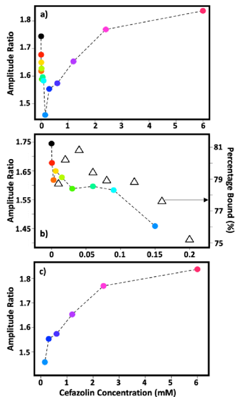
Figure 7. Amplitude ratio of 2D-IR spectra at points shown in Figure 6a,b as a function of cefazolin concentration. The ratio compares the high frequency point (1656, 1649 \text{cm}^{-1} ) to the lower frequency peak (1635, 1632 \text{cm}^{-1} ). (a) Amplitude ratio as a function of the full cefazolin concentration range studied. (b) The same results focusing on the 0–0.2 mM range. Hollow triangles show the percentage of cefazolin bound to HSA in serum as a function of cefazolin concentration from ref 30. (c) Amplitude ratio of samples containing more than 0.2 mM of cefazolin.
