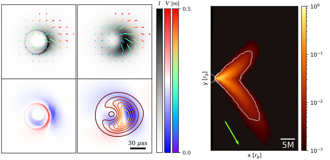
Figure 9. The best-fit model of Sgr A*: MAD a_* = 0.94 , R_{\text{high}} = 160 , i = 150^\circ aligned. In the left two columns, we plot its simulated image in the style of Figure 5. Images in the first column are unblurred, and images in the second column are blurred with a Gaussian with an FWHM of 20 \mu\text{as} , approximating EHT resolution. In the right panel, we provide a map of the emission in this model. The white contour encloses 90% of the total emission, the dashed white circle demarcates the horizon, and the green arrow indicates our viewing angle. While the emission peaks close to the BH in the midplane, a significant fraction of emission originates from a more diffuse region, including the jet sheath.
