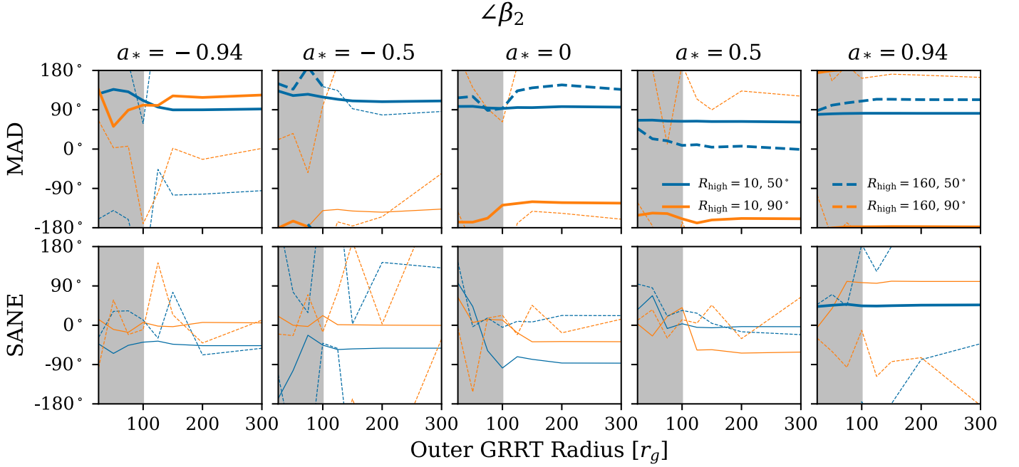
Figure 25. \angle\beta_2 as a function of outer integration radius for a selection of KCHARMA models. The GRRT in our work includes material at r \leq 100r_g , encoded by the gray band. Lines transition from thick to thin at the first radius at which |\beta_2| < 0.05 . For models with |\beta_2| > 0.05 , \angle\beta_2 typically converges by r = 100r_g .
