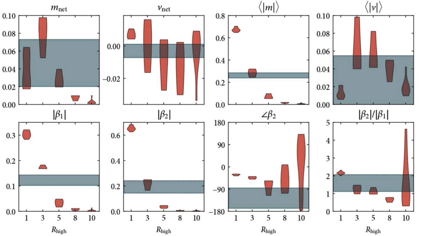
Figure 29. Distributions of observables for a selection of SANE models ray-traced with greater resolution in R_{\text{high}} between 1 and 10. These correspond to KCHARMA SANE a_* = -0.5 , i = 150^\circ aligned models. We find rapid evolution in this part of parameter space.
