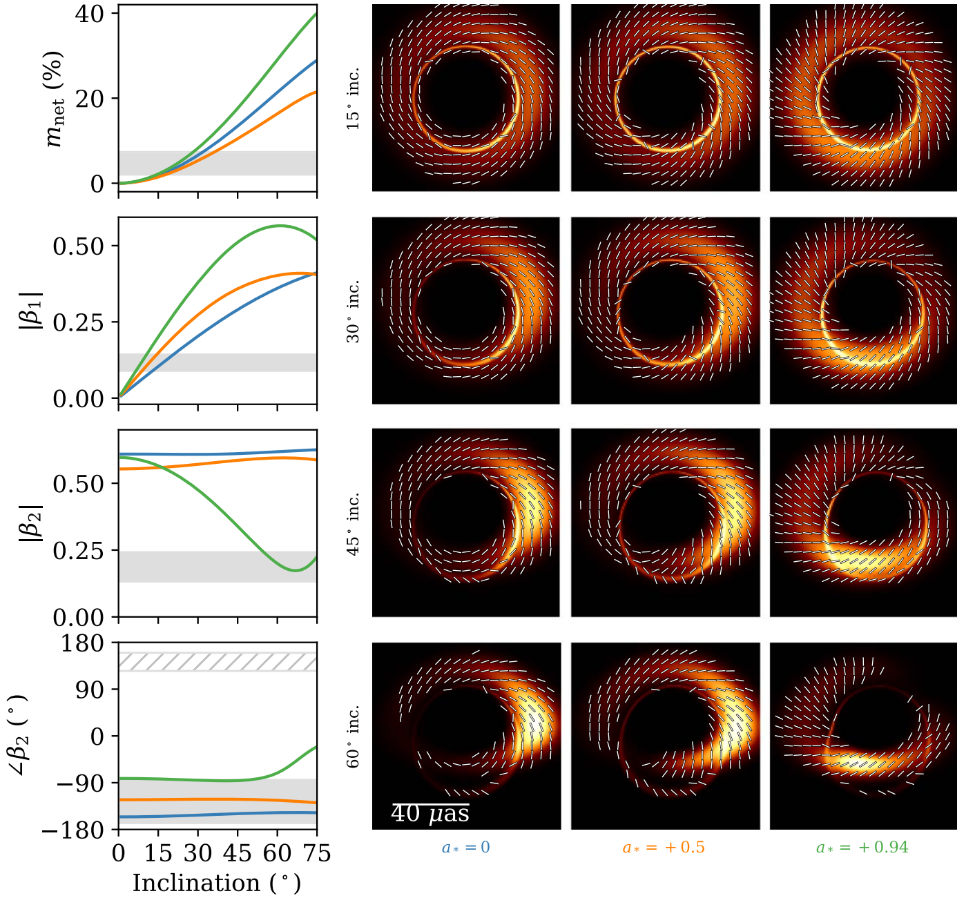
Figure 4. Left column: image quantities determined from simplified analytic KerrBAM models evaluated using MAD GRMHD fluid velocities and magnetic fields of three spins. In this and subsequent figures, we plot our observational constraints as gray bands for reference, with the \angle\beta_2 constraint prior to RM derotation shown as a hatched region. We use this model to understand key trends, but we caution that more physically complete GRMHD models are necessary for quantitative comparison. Right three columns: corresponding KerrBAM images evaluated at four example inclinations.
