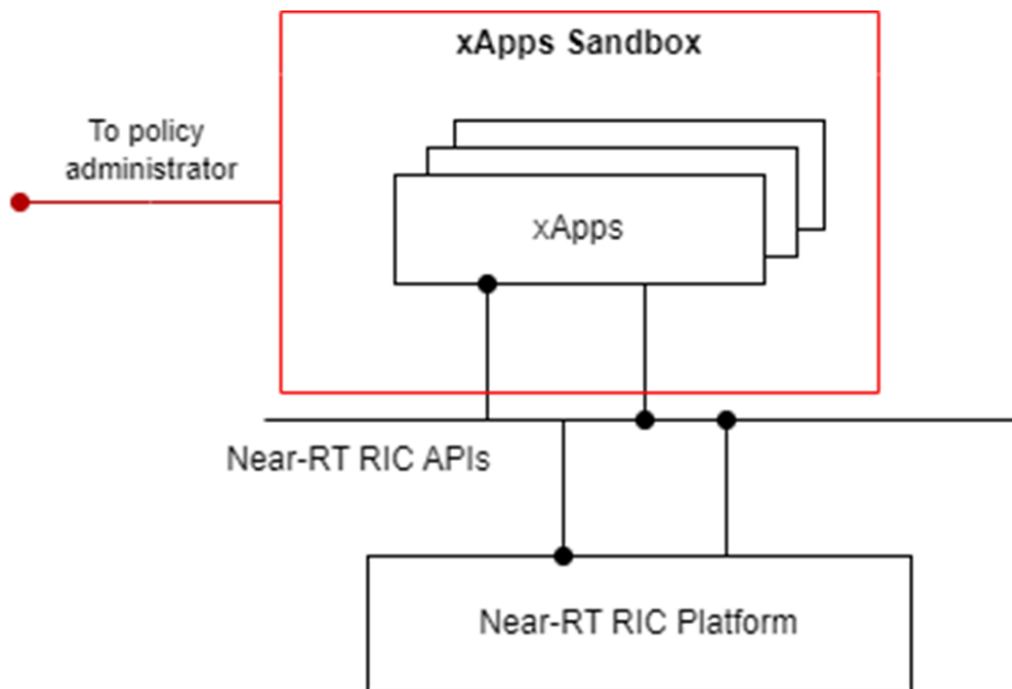
Figure 4. Sandboxed xApps.
